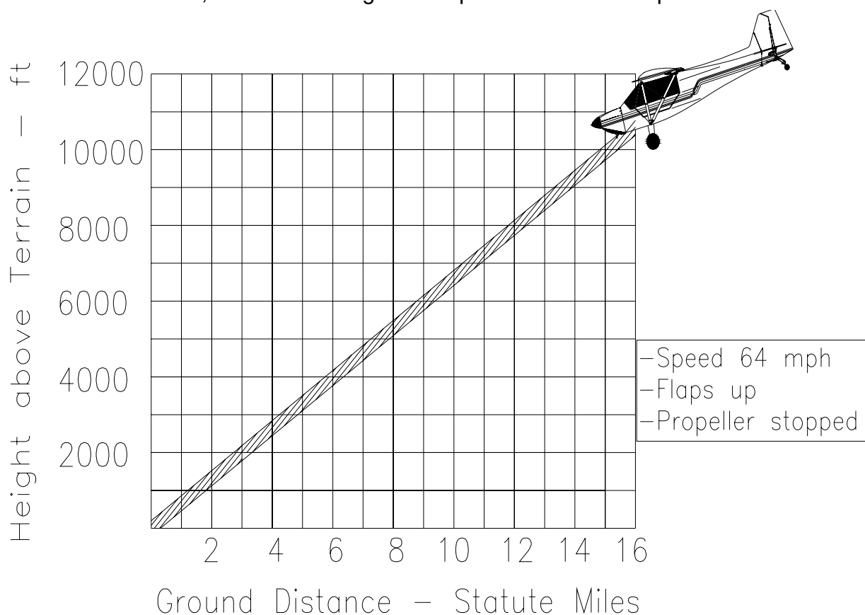
FIGURE 10-10. Maximum Glide
