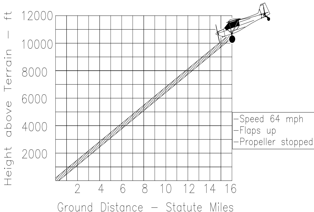
FIGURE 10-10. Maximum Glide
